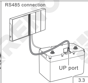
RS485 connection
